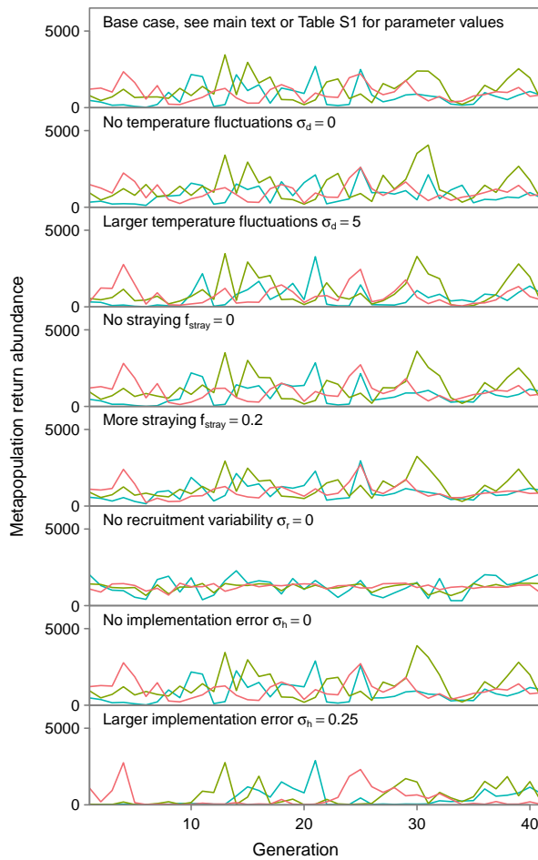
FIG. C1. The impact of increasing or decreasing various parameter values on metapopulation return abundance. The different coloured lines represent three example salmon populations. The base case represents the base-case values for the short-term environmental fluctuation scenario.
